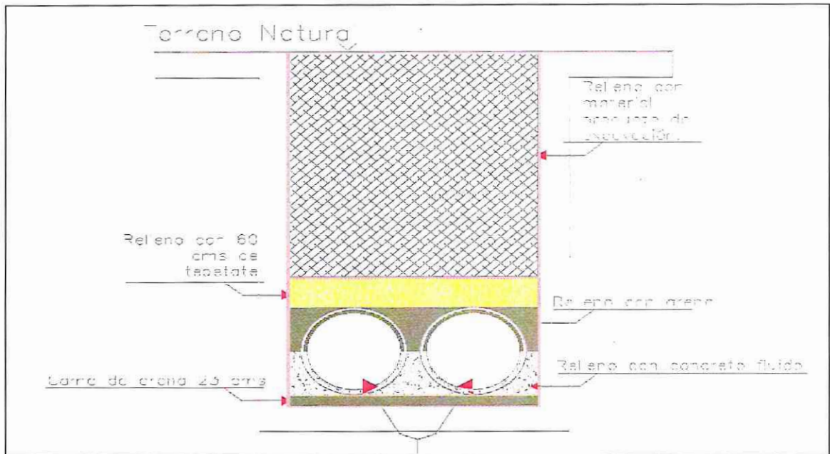
TUBERIA 60" PEAD
